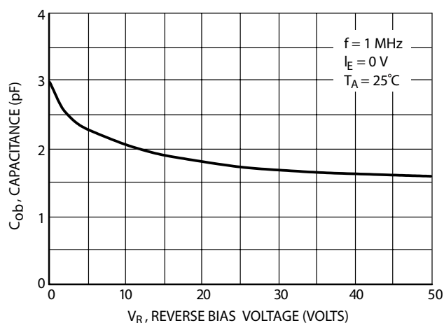
FIG.4 Output Capacitance
