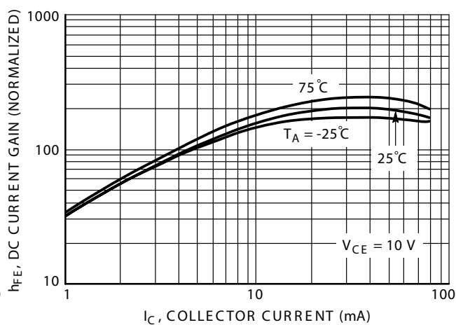
FIG.68 DC Current Gain
