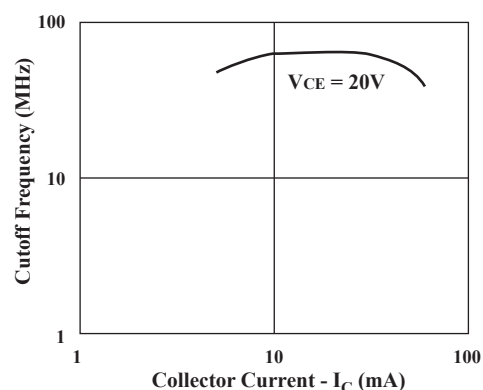
Fig.4 Cutoff Frequency & Collector Current
