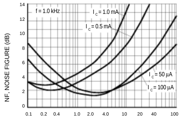
Figure 8. Noise Figure
