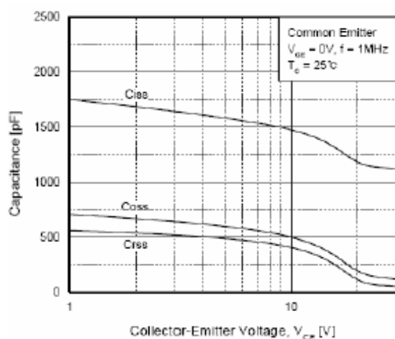
Fig.5 Capacitance Characteristics
