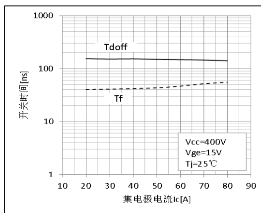
Figure 14.Switching Time -Ic Characteristics
