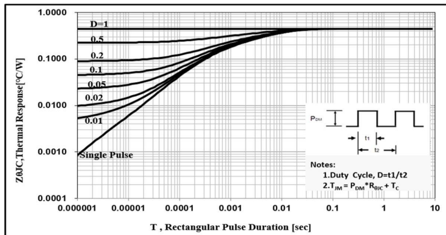
Figure 19.IGBT Transient Thermal Impedance
