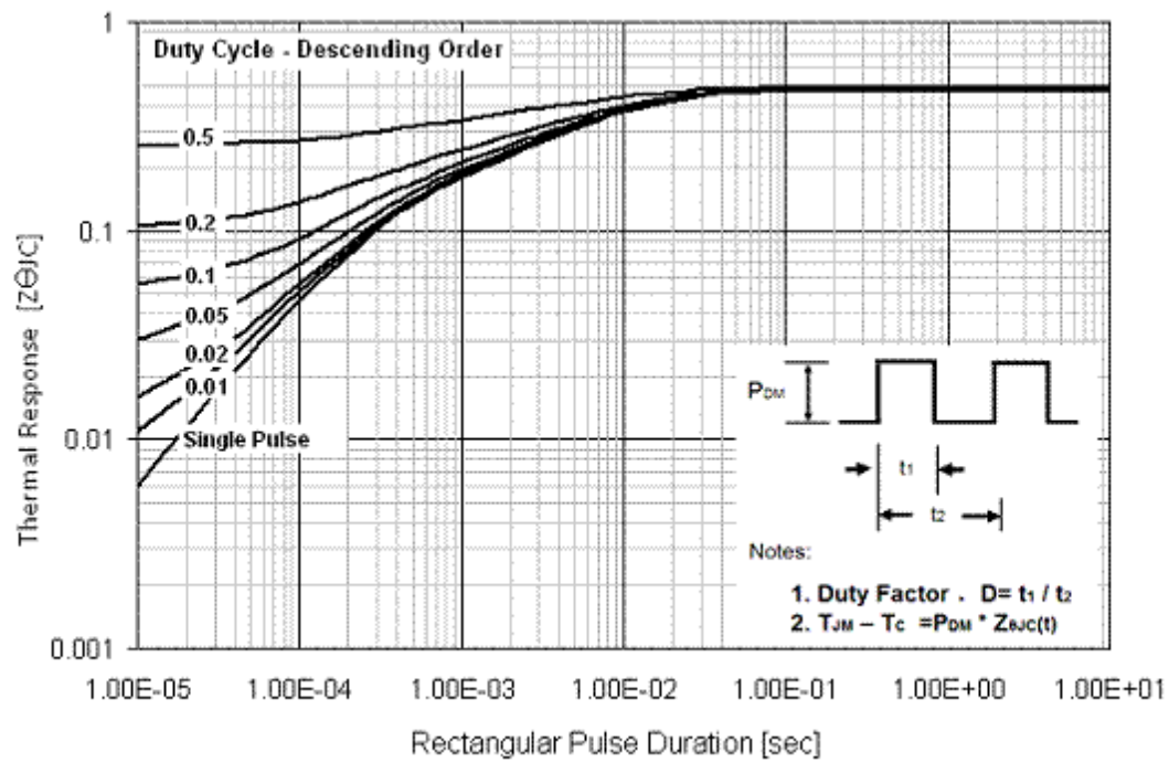
Figure 19.IGBT Transient Thermal Impedance
