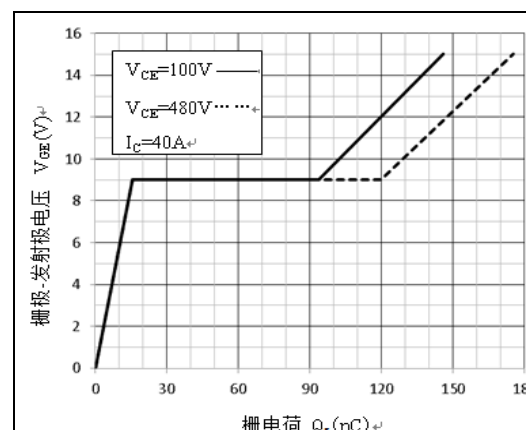
Figure 18.Gage Charge Characteristics
